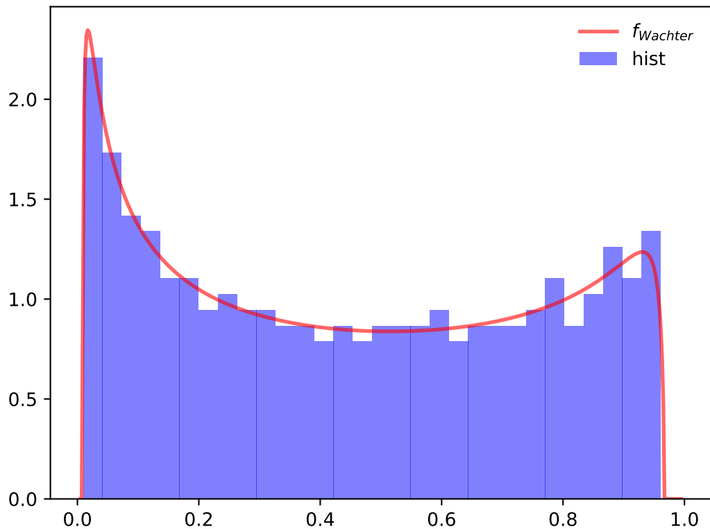
Realization of 400 points of Jacobi Ensemble with \beta = 2 with ratios, M_1/N \approx 1.250 , M_2/N \approx 1.500
