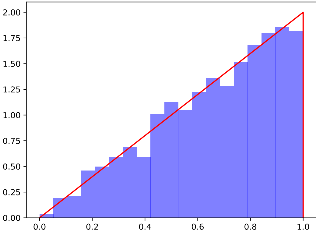
Realization of 1000 points of Ginibre Ensemble with \beta = 2 Histogram of the modulus of each points
