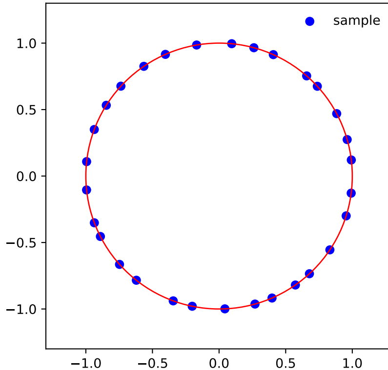
Realization of 30 points of Circular Ensemble with \beta = 5 using quindiang model
