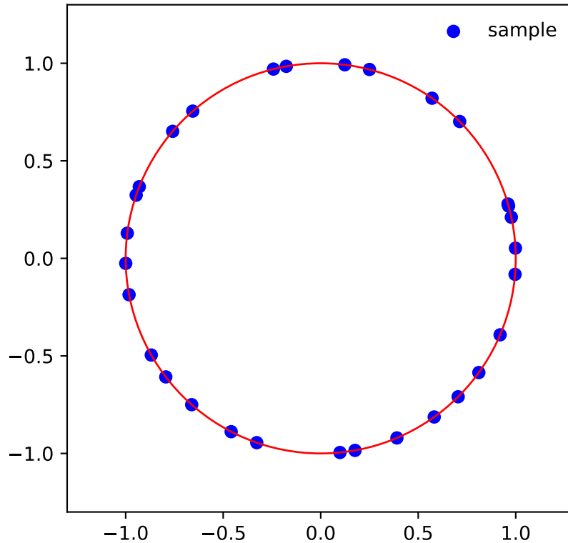
Realization of 30 points of Circular Ensemble with \beta = 1 using quindiang model
